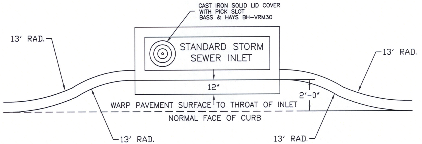
PLAN OF INLET
